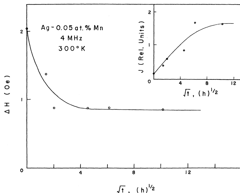
FIG. 4. Total linewidth \Delta H vs \sqrt{t} , where t is the running total of separate annealing times at 500 °C. The depth of internal oxidation is expected (Ref. 25) to be proportional to \sqrt{t} . The increase in peak-to-peak height J is also shown.
